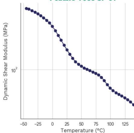
Dynamic Shear modulus-temperature Pebax® 7033 SP 01
