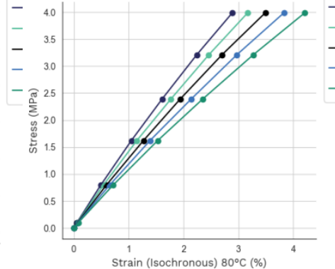
Stress-strain (Isochronous) 80°C Pebax® 7033 SP 01
